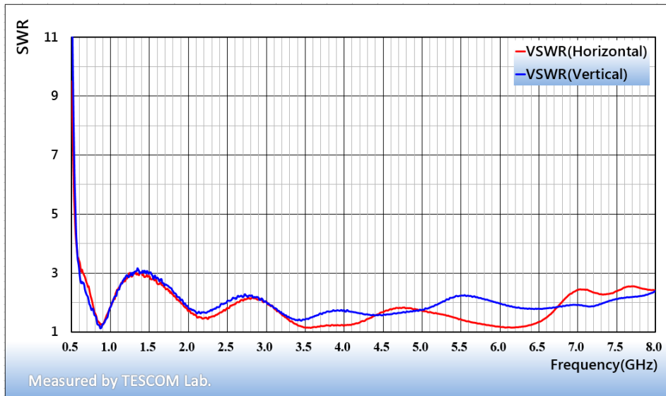
Graph1. TC-93083A VSWR
