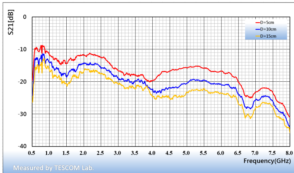
Graph2. TC-93083A Path-Loss(Horizontal)
