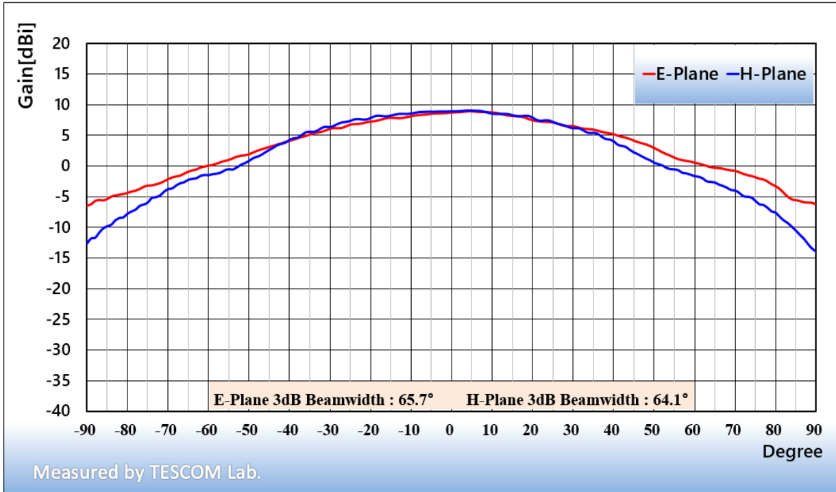
<TC-93473A @ 24 GHz>
