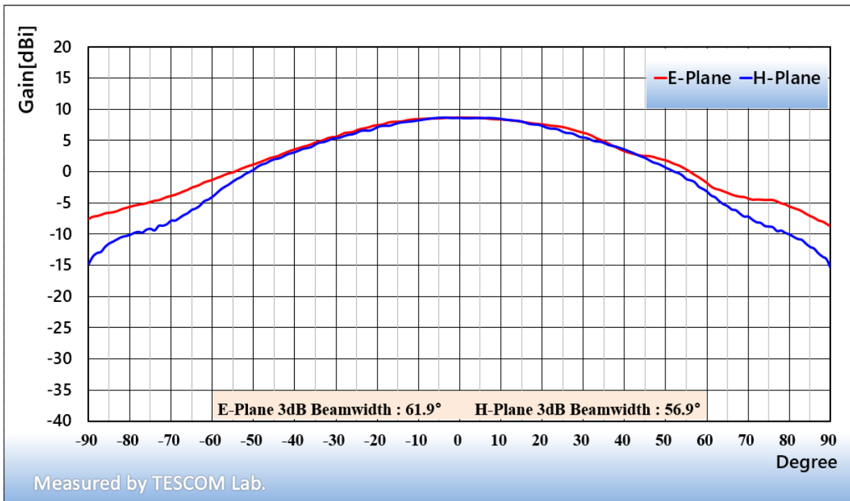
<TC-93473A @ 28 GHz>
